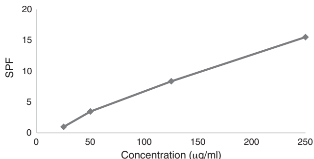
Fig. 2. Sun Protection Factor (SPF) of the ethanolic extract of Marcetia taxifolia .
