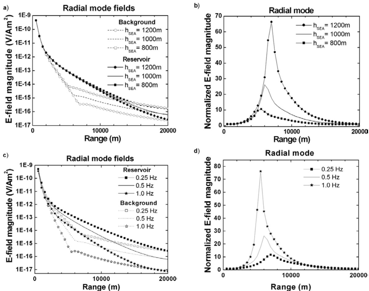
Figure 4 – Results from the model with the different deep water layers and different frequencies; (a,c) Electric field magnitude for the Radial mode; (b,d) Normalized field in the Radial mode.
