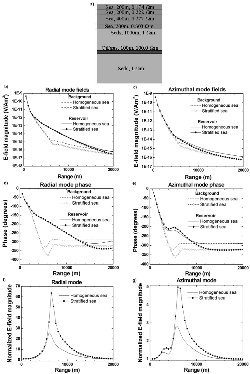
Figure 3 – Results from the model with the non homogeneous sea water with four layers, at a frequency of 0.5Hz. (a) Model; (b,c) Electric field magnitude for the Radial and Azimuthal mode; (d,e) Phase in the Radial and Azimuthal mode; (f,g) Normalized field in the Radial and Azimuthal mode.
