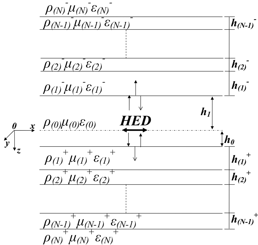
Figure 1 – Model with the non homogeneous water layer.
