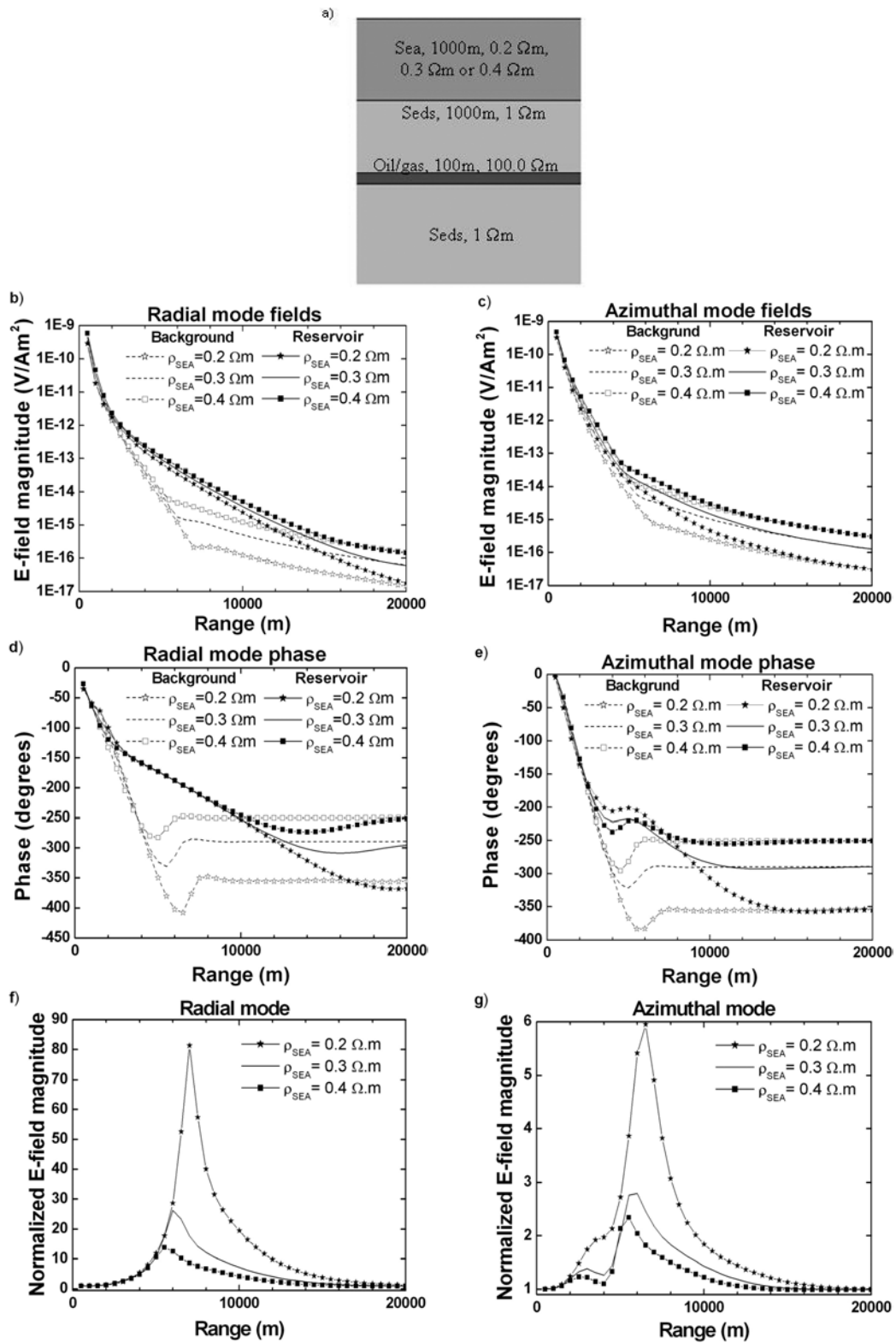
Figure 2 – Results from the model with one homogeneous water layer, at a frequency of 0.5Hz. (a) Model; (b,c) Electric field magnitude for the Radial and Azimuthal mode; (d,e) Phase in the Radial and Azimuthal mode; (f,g) Normalized field in the Radial and Azimuthal mode.
