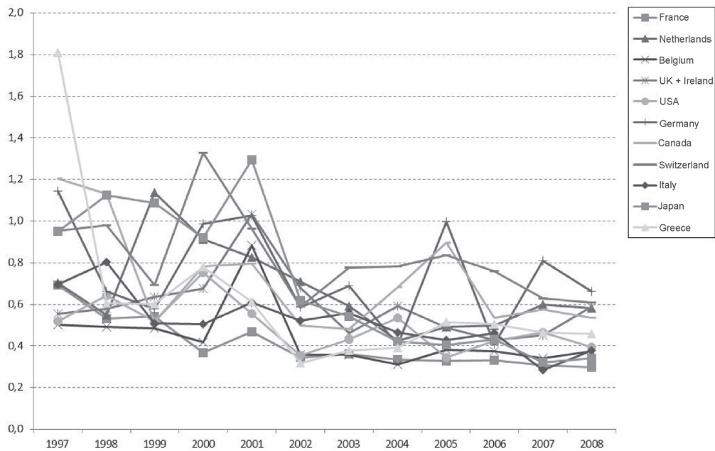
FIGURE 3 – Evolution of the beta-convergence of Y_1
