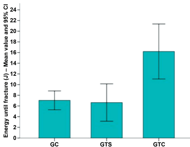
Fig. 6 Mean energy until fracture and 95% confidence interval (CI).
