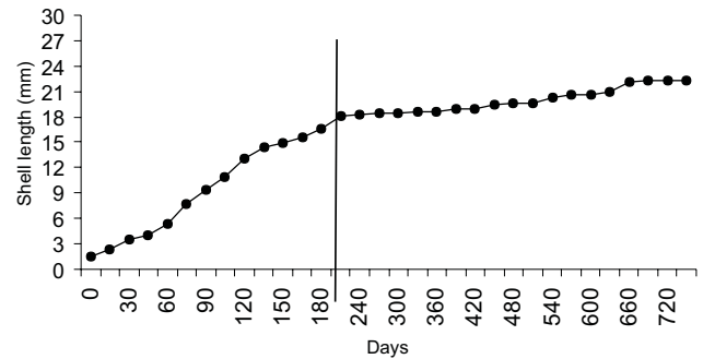
Figure 1. Snail growth during the study. Points show average shell length (mm) for Bulimulus tenuissimus in the grouped treatment for two years. Vertical line shows when egg laying began.
