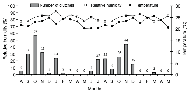
Figure 2. Average temperature and relative humidity and number of clutches laid each month by Bulimulus tenuissimus in groups from August 2005-May 2007. Numbers above bars indicate the number of clutches.
