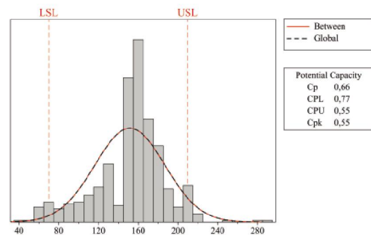
Figure 3 - Analysis of the effective seed-spacing capacity
