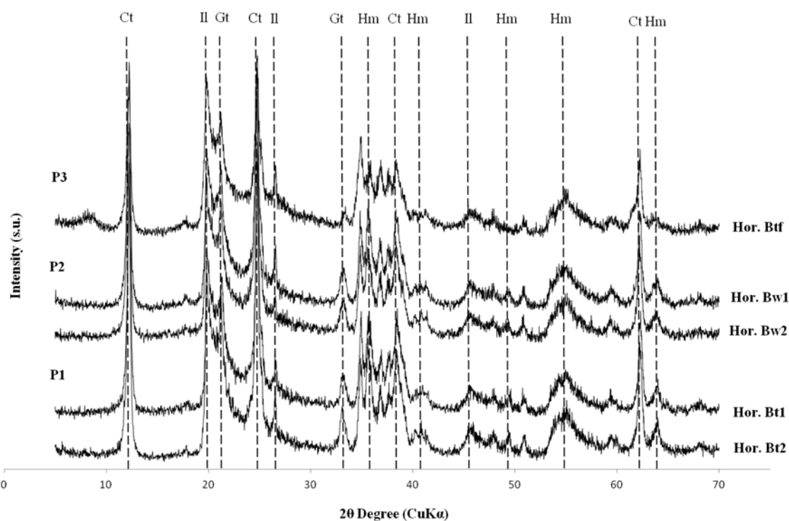
Figure 2. X-ray diffractometry (XRD) the clay fraction profiles of diagnostics horizons in: Typic Rhodustults (P1); Rhodic Haplustox (P2) e Typic Plinthustalfs (P3). Ct: kaolinite; Il: Illite; Gt: Goethite; Hm: Hematite.
