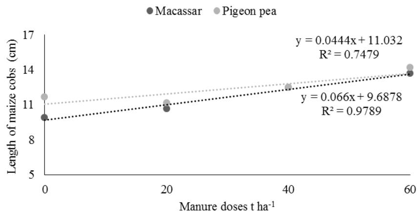
Figure 1. Length of maize cobs as a function of the doses of cattle manure associated with green manure, Macassar and Pigeon pea beans.
