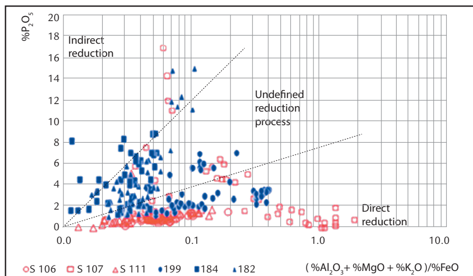
Figure 3 Graph showing the content of %P 2 O 5 versus the [(%Al 2 O 3 + %MgO + %K 2 O) / %FeO] ratio found in the slag inclusions of each iron artefact of both production sites of Ara- çoabi Hill (S: Sardinha and I: Ipanema).
