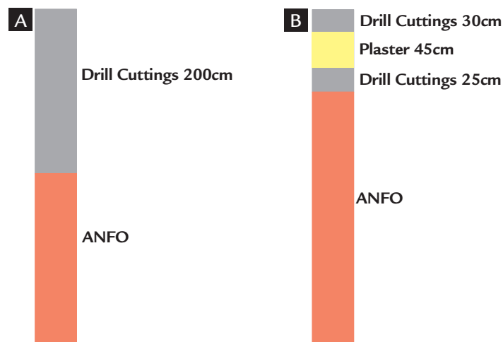
Figure 5 Blast hole Stemming at Gumusgun limestone quarry. (A) Stemming with drill cuttings. (B) Stemming with plaster.
