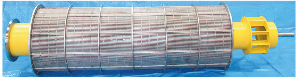
Figure 6 Rotor Matrix Assembly
