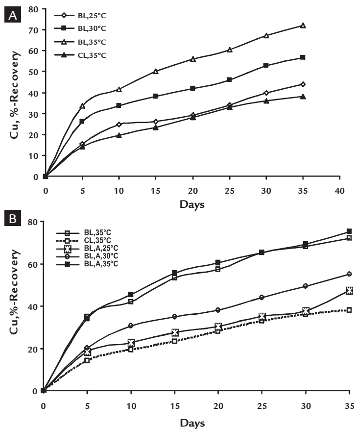
Figure 3 Effect of temperature on copper bio-recovery with culture of (A) un-adapted and (B) adapted bacteria [Particles: <math><50\mu\text{m}</math>, 2.0 pH, Pulp density: 5% (w/v)].
