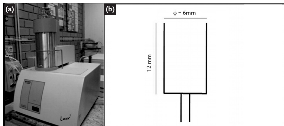
Figure 1 a) Thermobalance (LaSid - UFRGS) and b) Crucible used for the tests.
