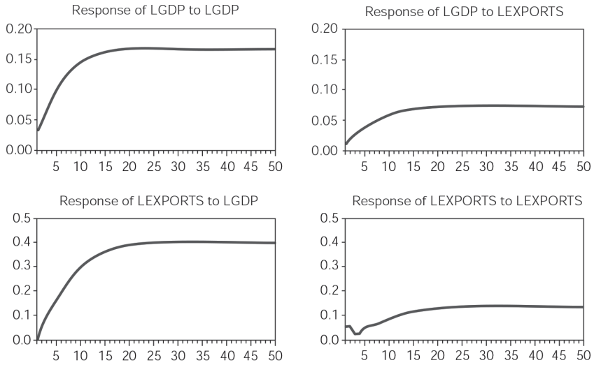
Figure 2: Response to Innovations to One S tandard Deviation Response to One S .D. Innovations
