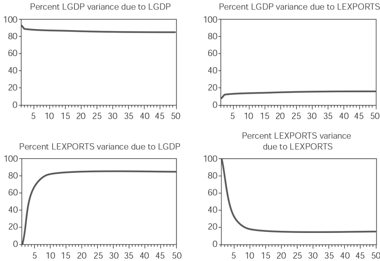
Figure 3: Variance Decomposition
