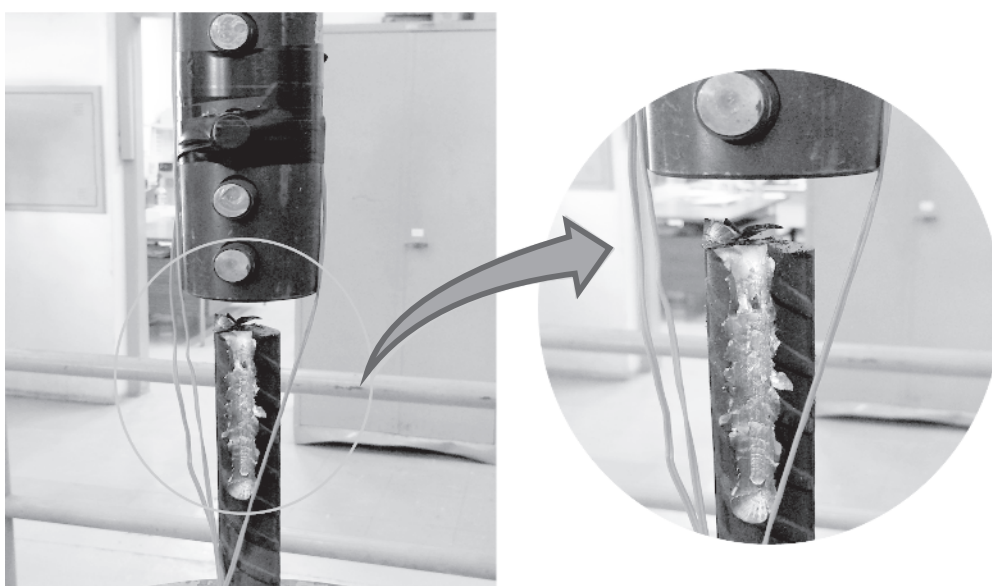
Figure 18 Detailed view post-rupture of spliced bar with shear bolted coupler
