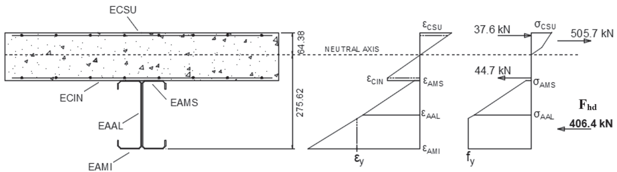
Figure 10 Resultant force F_{hd} for applied load of 137.3 kN on Specimen 01 obtained from strain gauges
