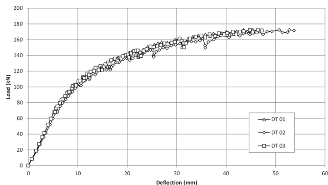
Figure 7 Load (kN) x vertical deflection (mm) under the loading points (DT 01 e DT 03) and on the central section (DT02) of Specimen 01
