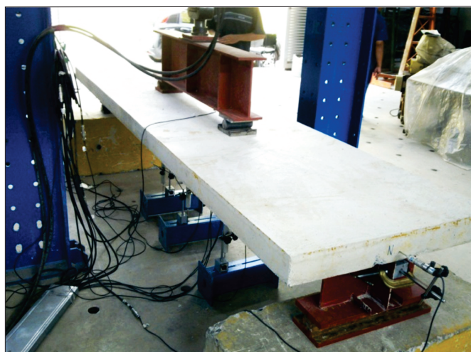
Figure 5 Experimental set-up
