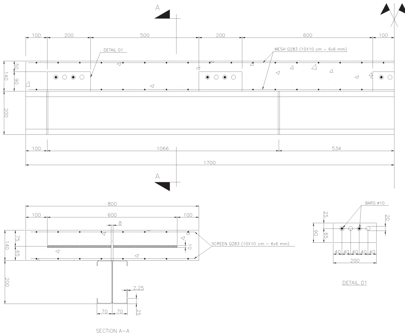
Figure 4 Geometry of the specimens, sizes in millimeters
