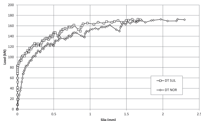
Figure 8 Load (kN) x slip (mm) on steel - concrete interface, at the ends of Specimen 01
