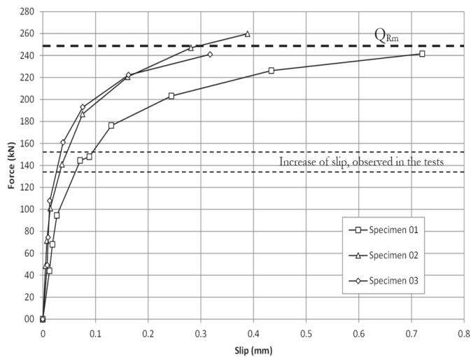
Figure 11 Force (kN) x slip (mm) curves of the connector
