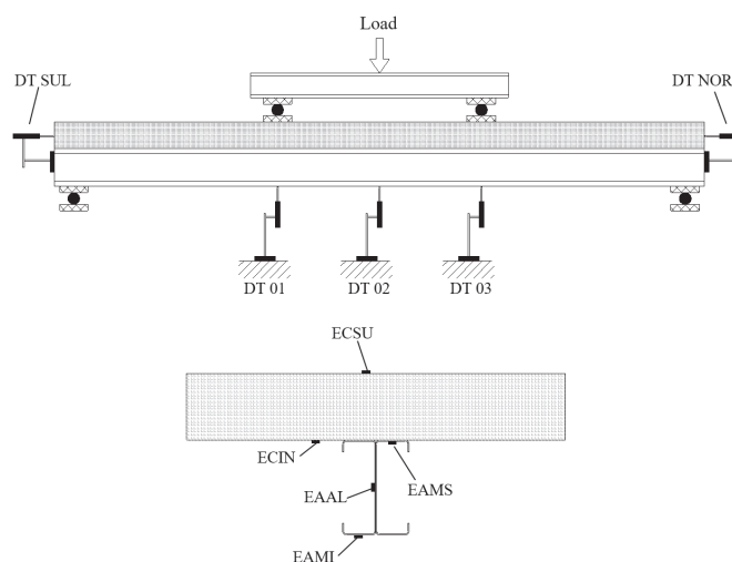
Figure 6 Strain gauges and displacement transducers
