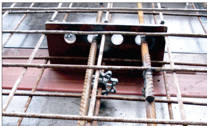
Figure 3 Tested connector prior to concrete casting
