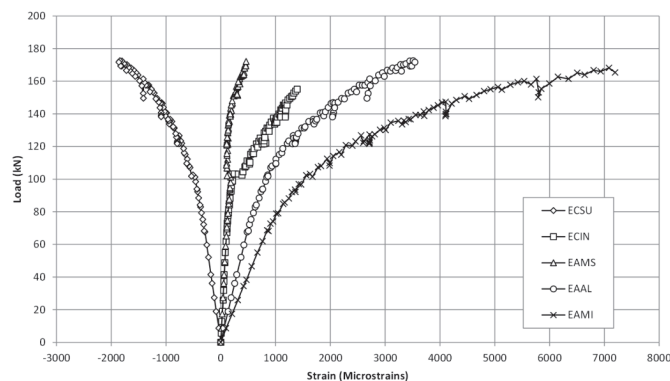
Figure 9 Load (kN) x strain (10 -6 ) at various points of the mid-section of Specimen 01
