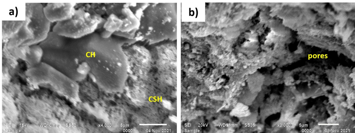
Figure 7. SEM micrograph of a concrete sample heated to a temperature of 800°C: a) less degraded sample; b) most degraded sample.
