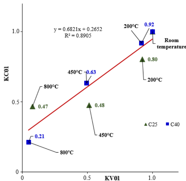
Figure 5. Correlation curve of KC \theta 1 versus KV \theta 1 for C25 and C40.
