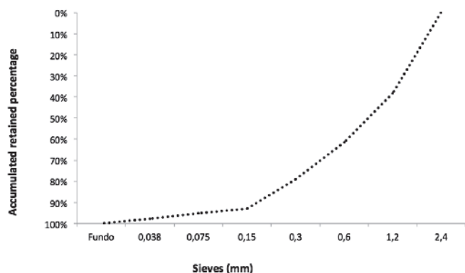
Figure 11 Granulometric distribution used to mortar production with different crushed aggregates
