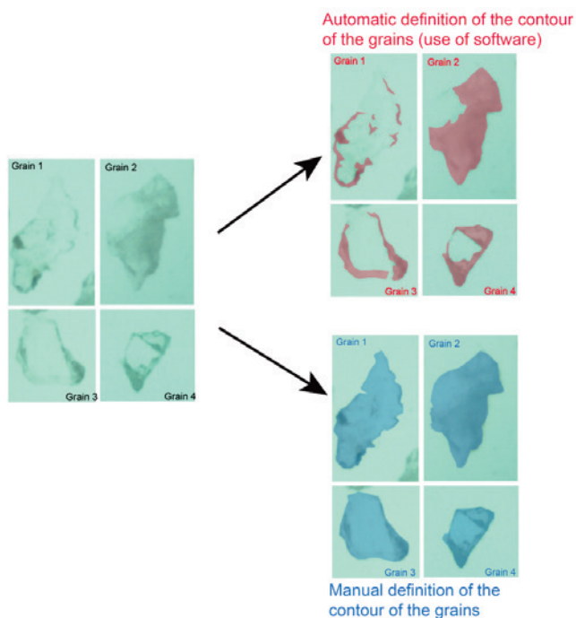
Figure 7 Detail of the automatic and manual obtainment of the contour of the grains (passing material in the 0.075 sieve)
