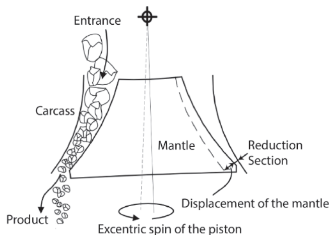
Figure 2 Details of the functioning of the conic crusher (adapted from Itävuo et al. [8])
