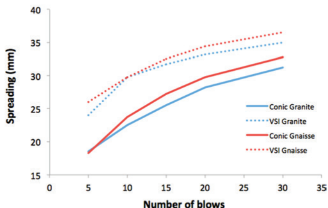
Figure 12 Results of spreading by the number of blows applied for the crushed fine aggregates employed in the present study
