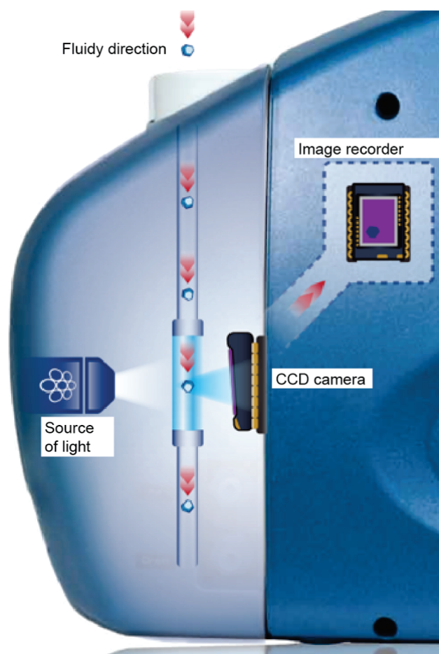
Figure 8 Detail of functioning of the analyzer of dynamic images of particles (adapted from Ulusoy&Yekler[25])
