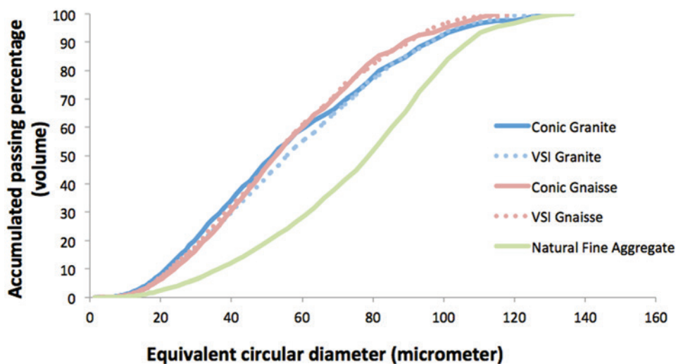
Figure 9 Granulometric distribution of the passing particles in the sieve of 0.15 mm opening
