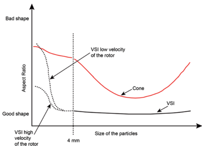
Figure 4 Aspect ratio form crushed aggregates from VSI crushers (high and low velocities of the rotor) and conic crushers (adapted from Bengtsson et al. [14])
