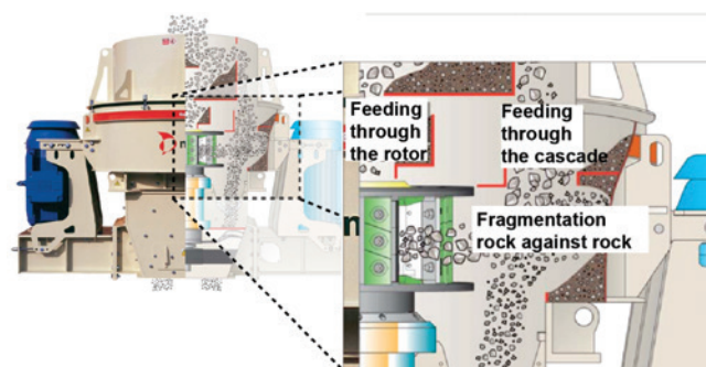
Figure 1 Detail of functioning of the VSI crusher (adapted from Metsominerals [4])
