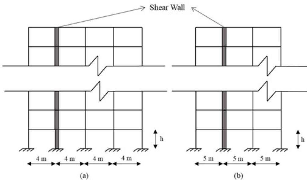
Figure 2. Frames models: dual system structures.
