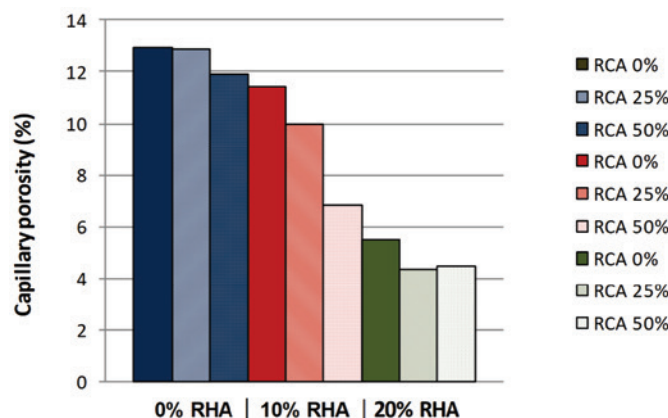
Figure 4 Capillary porosity on day 28
