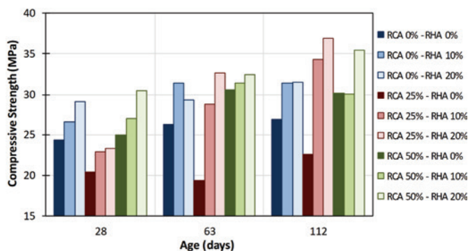
Figure 9 Compressive strength
