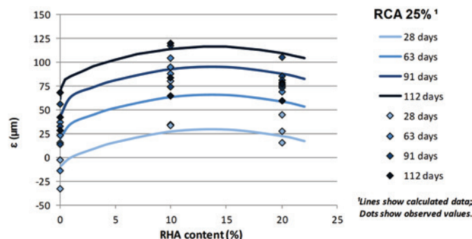
Figure 7 Shrinkage test, replacement with RHA with 25% RCA for mixtures of different ages
