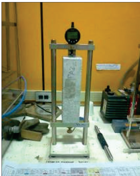
Figure 2 Equipament to measure length variation
