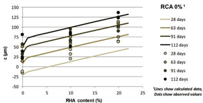
Figure 6 Shrinkage test, replacement with RHA with 0% RCA for mixtures of different ages
