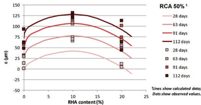
Figure 8 Shrinkage test, replacement with RHA with 50% RCA for mixtures of different ages
