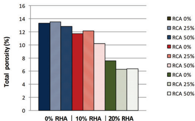
Figure 5 Total porosity on day 28
