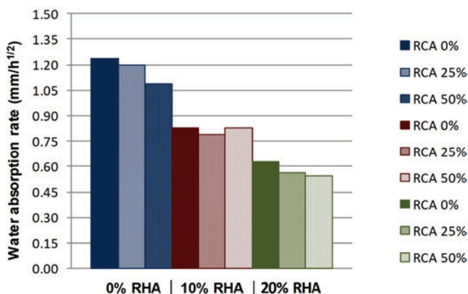
Figure 3 Absorption rate on day 28
