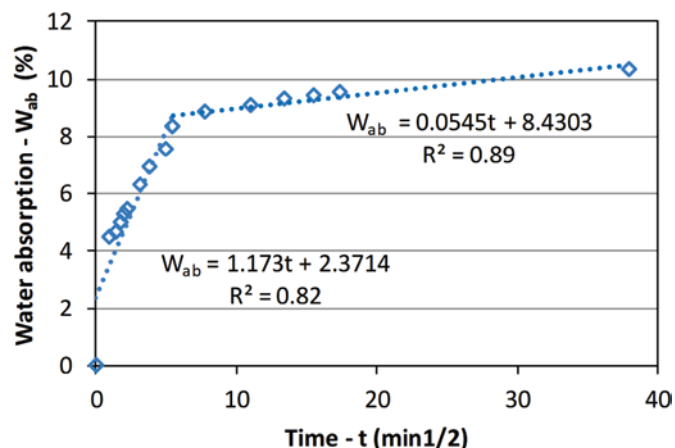
Figure 1 Water absorption curve of the recycled concrete aggregate
