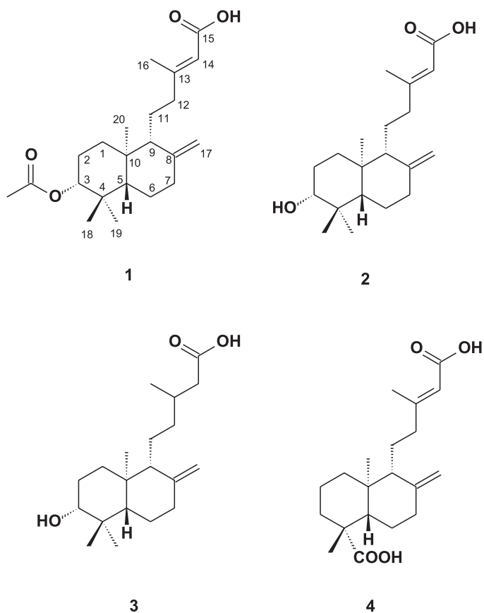
Fig. 1 - Structures of diterpenoids 1-4 . Diterpenoids 1 [(-)-3 \beta -acetoxylabdan-8(17)-13-dien-15-oic acid]; 2 {alepterolic acid [(-)-3 \beta -hydroxylabdan-8(17)-13-dien-15-oic acid]}; 3 [(-)-3 \beta -hydroxylabdan-8(17)-en-15-oic acid] and 4 ( ent -agatic acid).
