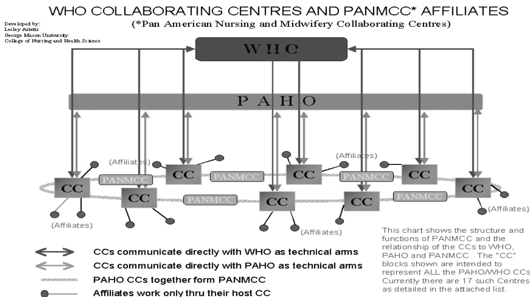
Figure 2 – Relationship of the Collaborating Centres to WHO and PAHO
