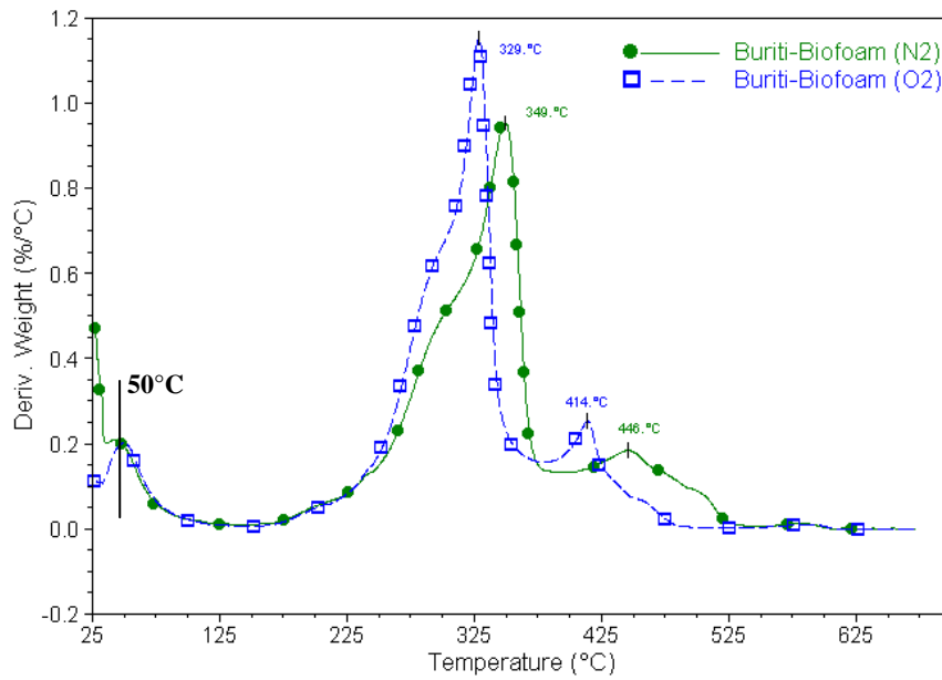
Figure 5: DTG curves for the buriti biofoam.
