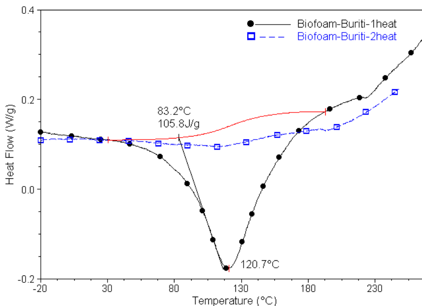
Figure 6: The DSC curve for the buriti biofoam heated under N2 atmosphere.
