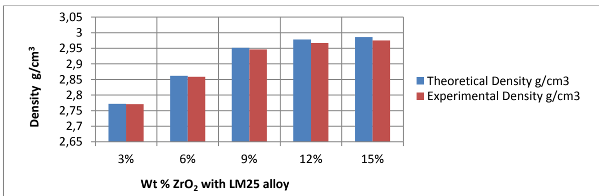
Figure 2: Comparisons of Theoretical and Experimental density
