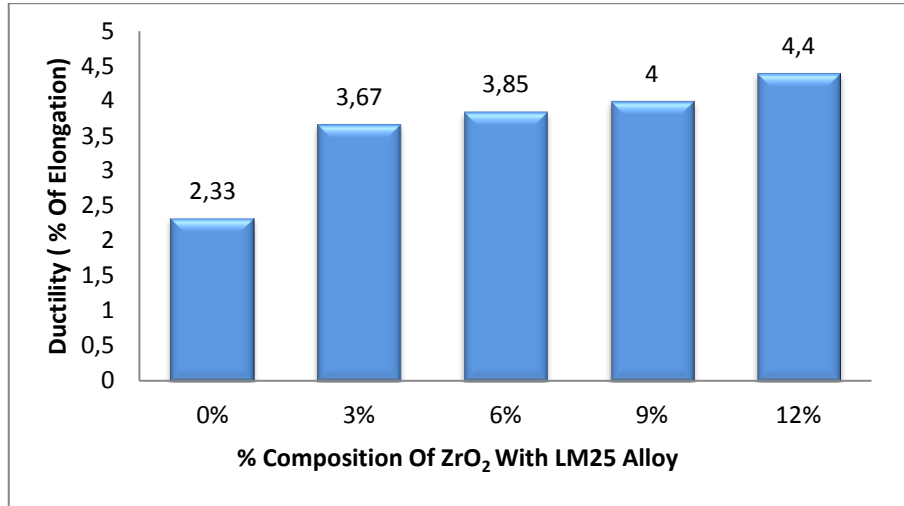
Figure 7: Variation in Ductility with wt% of ZrO_2 for LM25/ ZrO_2 Composites
