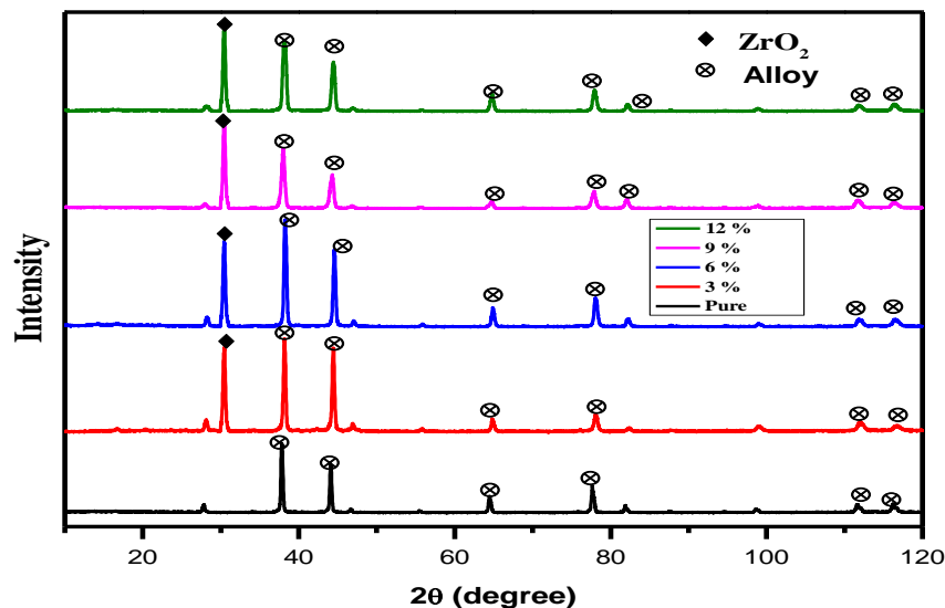
Figure 10: X-ray diffraction patterns of the specimen for LM25 with various wt% reinforcement of ZrO_2 Table 4 Peak position of LM25/ ZrO_2 composites.
