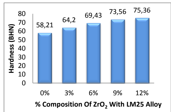
Figure 6: Hardness value with varying wt% of ZrO_2
