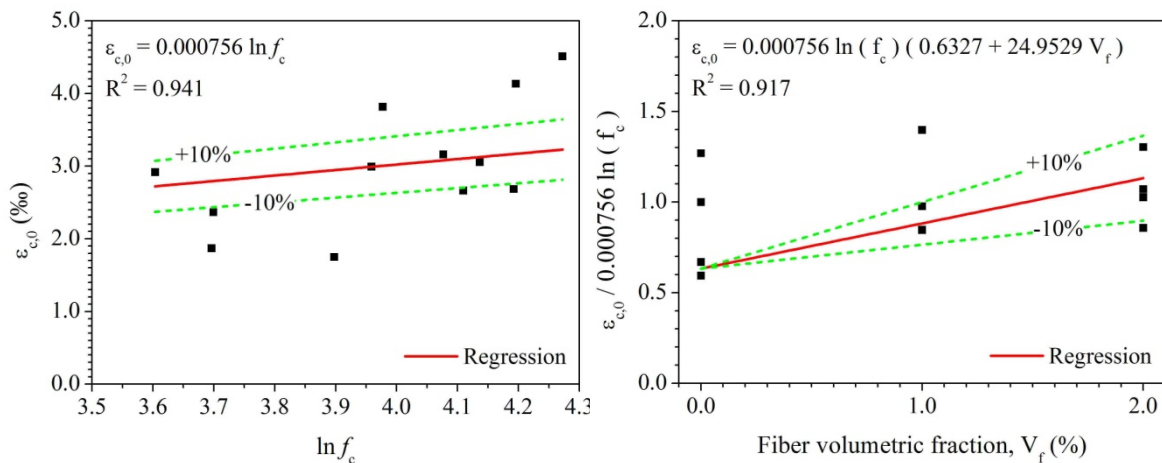
Figure 2: Regressions to define equation to estimate the peak strain.
