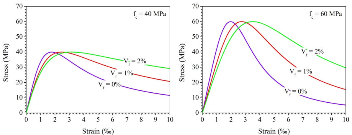
Figure 4: Analytical curves for concretes of 40 MPa and 60 MPa.
