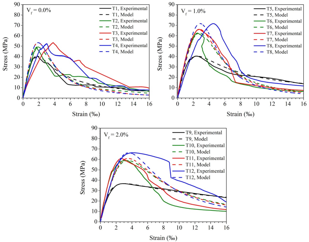
Figure 3: Comparison between experimental and analytical results.
