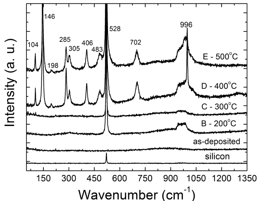
Figure 2: Raman spectra obtained for the as-deposited and thermally treated vanadium oxide films at various temperatures. The spectrum of the (100) silicon substrate is also presented.
