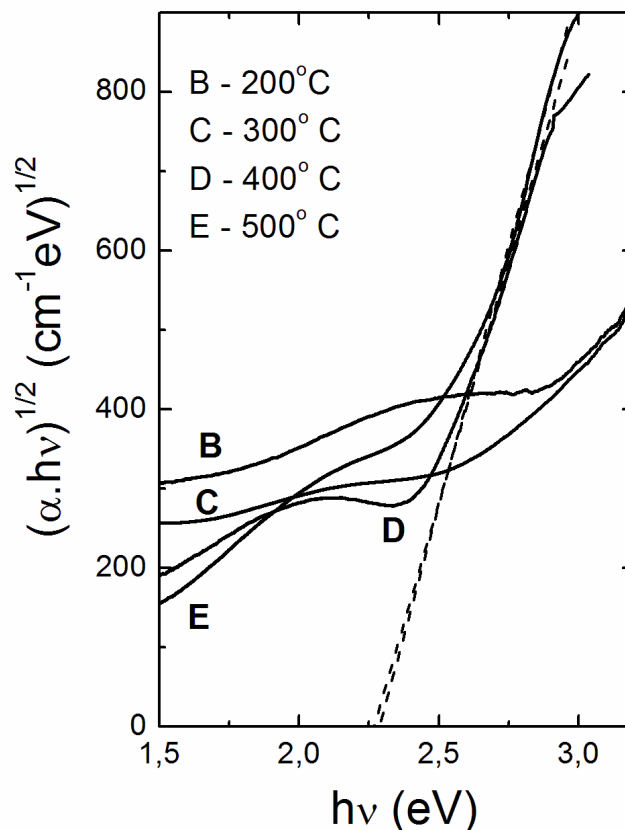
Figure 5: (\alpha h\nu)^{1/2} as a function of incident photon energy for vanadium oxide films annealed at the temperatures indicated in the top left corner. The dashed line is a fit of the linear part of the optical absorption edge for D and E films.
