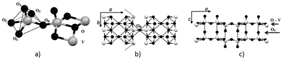
Figura 4: Vanadium coordination in a perfect V_2O_5 lattice (a); projection of the (010) planes of the V_2O_5 lattice, in which the zigzag dotted lines indicate the oxygen pyramids pointing alternatively up ( O_A atom visible) and down (V atom visible) in b direction (b); projection of the (001) planes (c).
