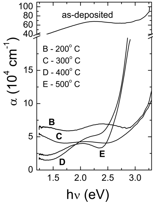
Figure 3: Optical absorption coefficient \alpha as a function of incident photon energy for as-deposited and for thermally-treated vanadium oxide films at various temperatures.
