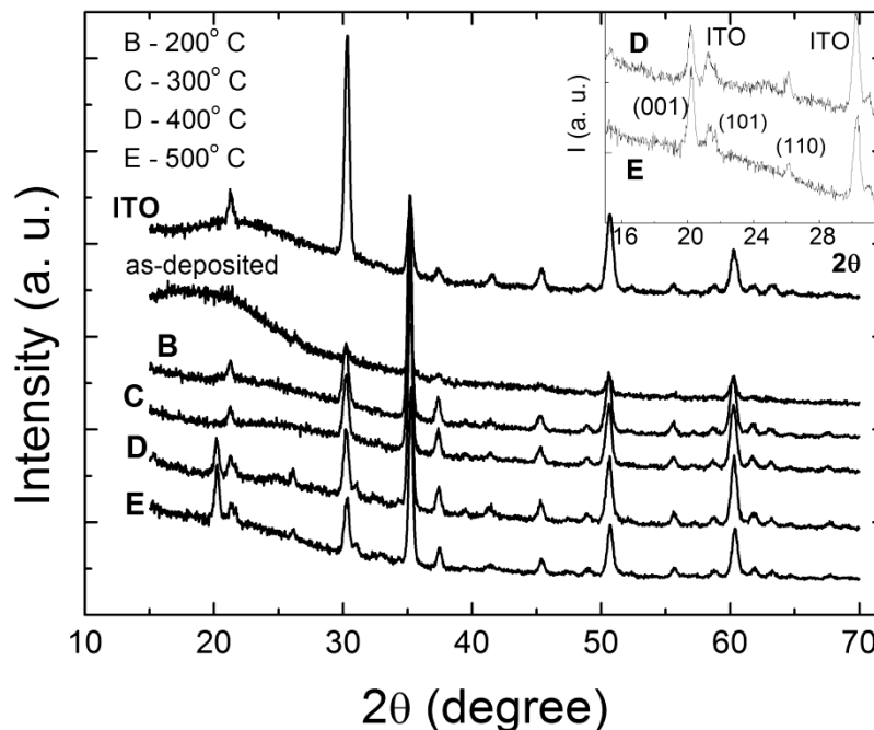
Figure 1: X-ray diffractograms for as-deposited and annealed vanadium oxide films. The inset shows the diffractograms for the D and E polycrystalline vanadium oxides. The diffractograms of the ITO layer x-ray is also shown.
