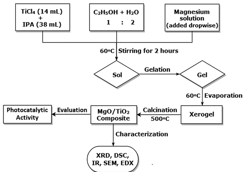
Figure 1: Flow diagram for the synthesis of MDT samples.
