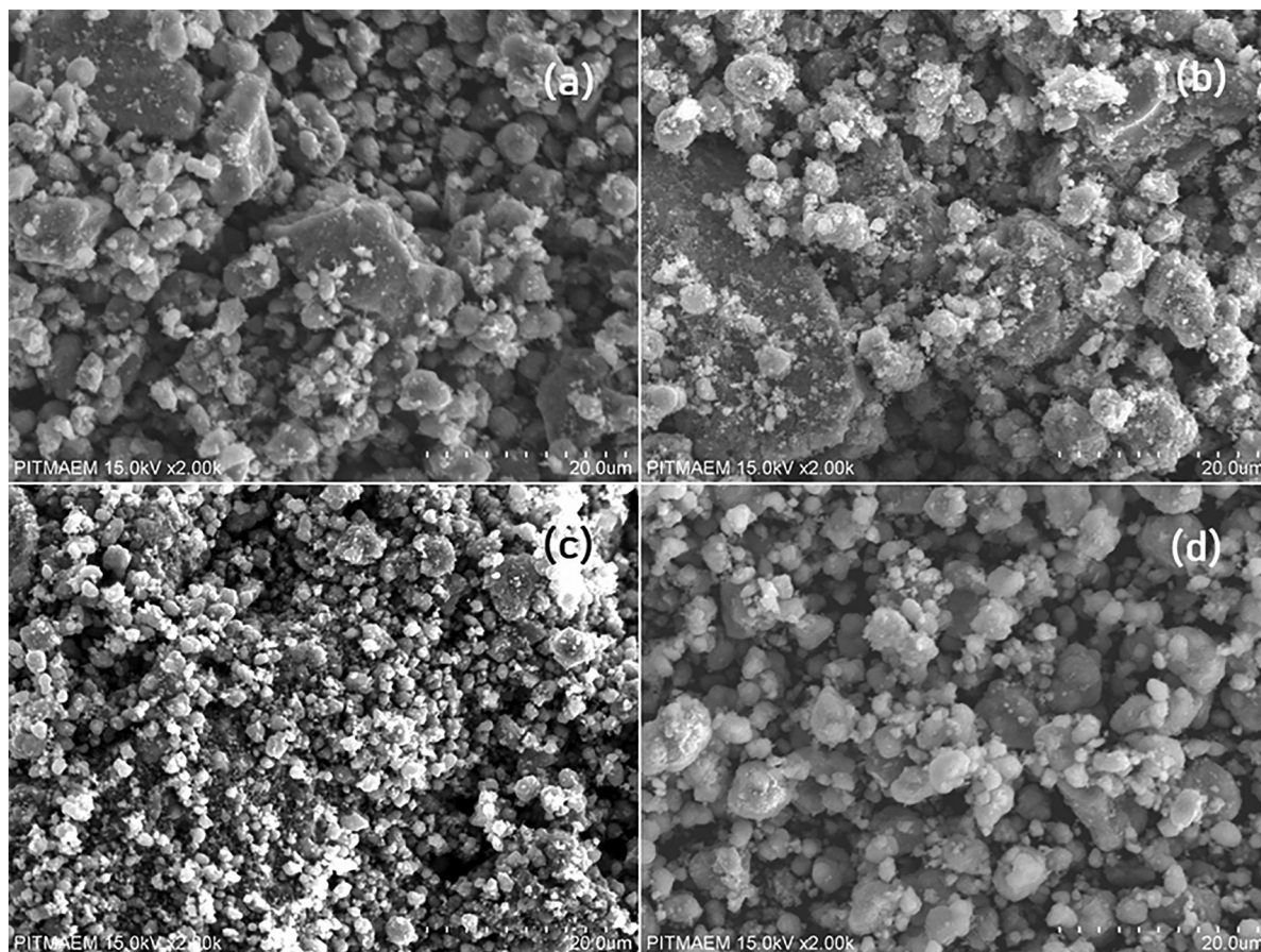
Figure 5: SEM micrographs (a) MDT-1; (b) MDT-2; (c) MDT-3; (d) MDT-4.
