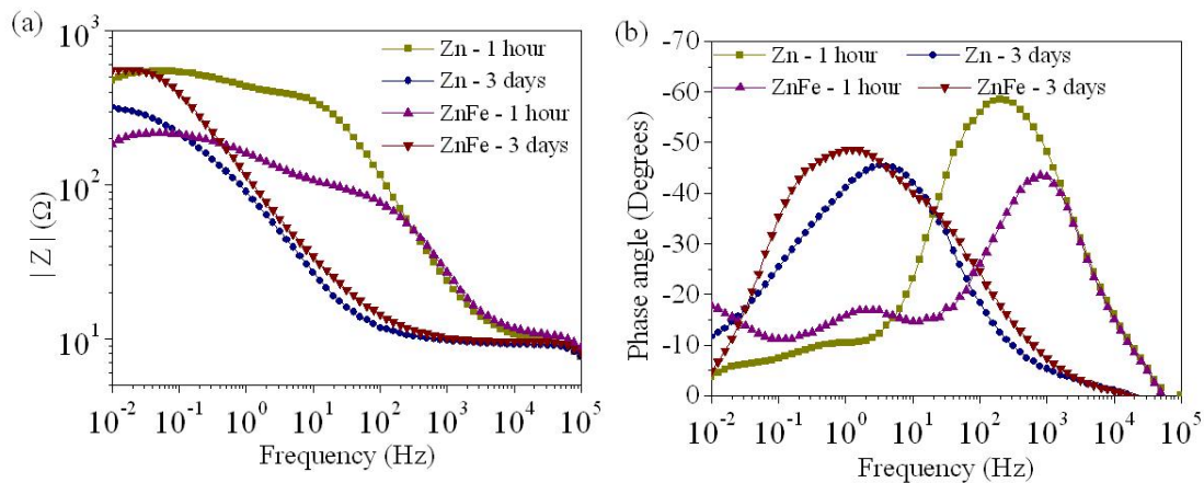
Figure 4: Bode Plots of Zn and ZnFe specimens at different times of immersion.
