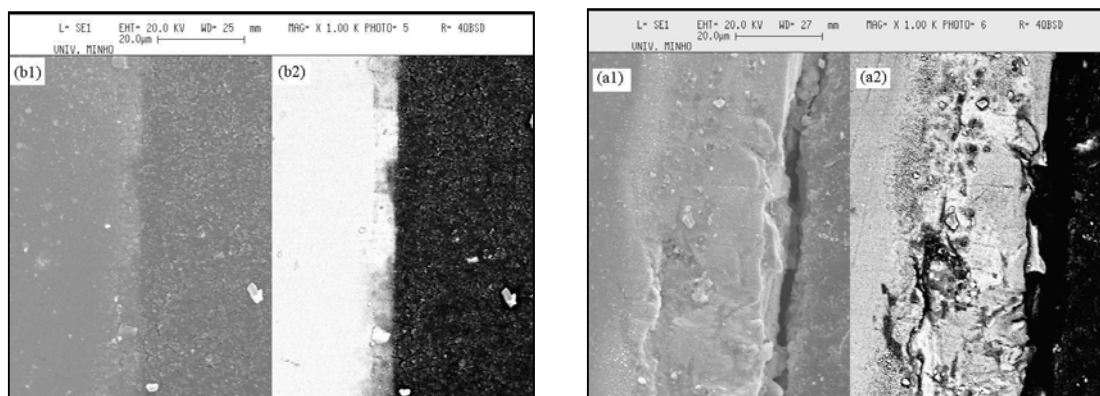
Figure 9: SEM micrographs of the cross section of Zn/R (a) and ZnFe/R (b). 1- Image of secondary electrons. 2- Image of back-scattered electrons.
