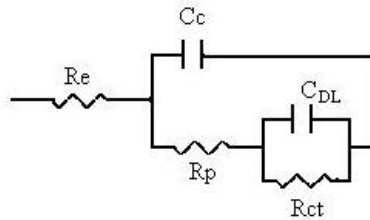
Figure 3: Equivalent electrical circuit
