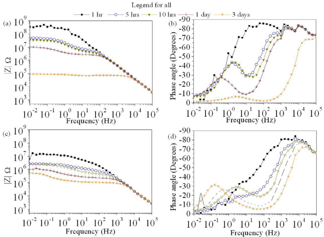
Figure 5: Bode plots of specimens Zn/R (a - b) and ZnFe/R (c - d) at different immersion times.
