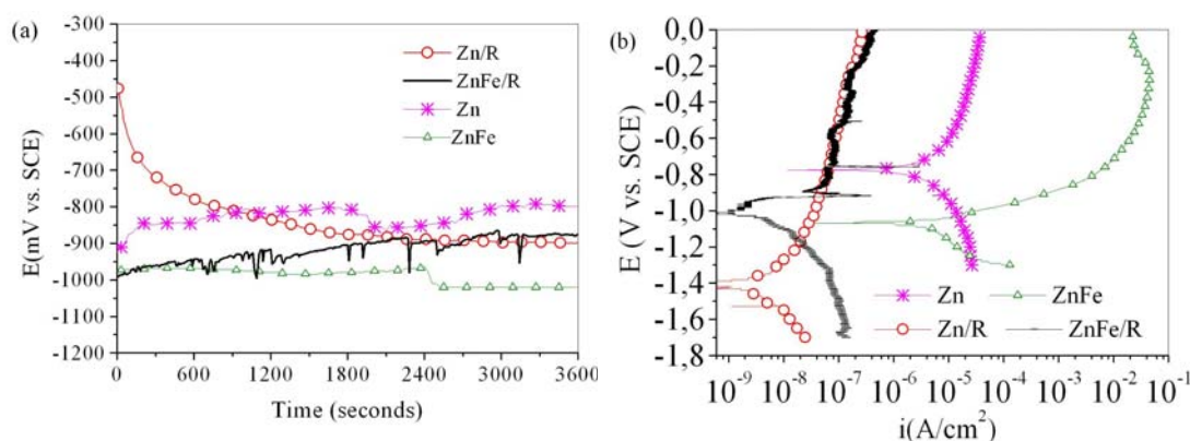
Figure 2: Open circuit potential and polarization curves of uncoated samples and resin-coated systems.
