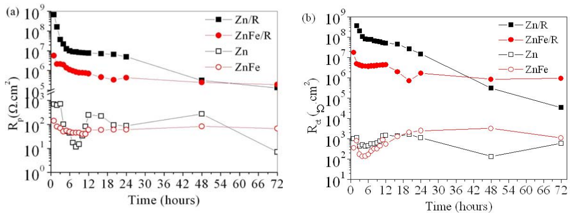
Figure 7: Time dependence of the coating pore resistance ( R_p ) and charge-transfer resistance ( R_{ct} ), for all samples in a 3% NaCl solution.
