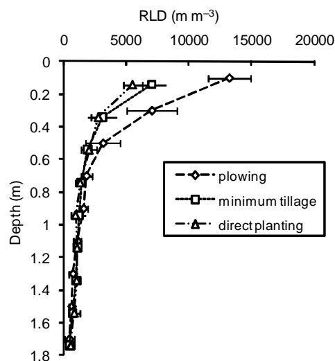
Figure 5 – Mean profiles of root length density (RLD) obtained 60 DAR according to three soil managements using the root intersection (RIC) method. The averages were calculated from 0.2 m depth \times 1.4 m long soil layers.
