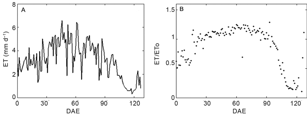
Figure 6 – (A) Seasonal distributions of evapotranspiration, and (B) variation of the daily crop coefficient K_c for the 2009/2010 soybean growing season.
