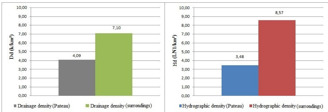
Charts 1 and 2 – Hydrographic density and drainage density average values.
