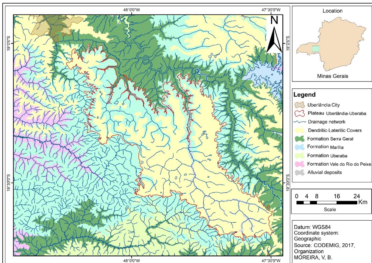
Figure 1 – Uberlândia-Uberaba plateau and surroudings litostratigraphic units.
