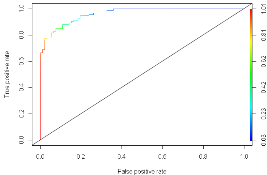
Figure 12- ROC curve for LR Model.
