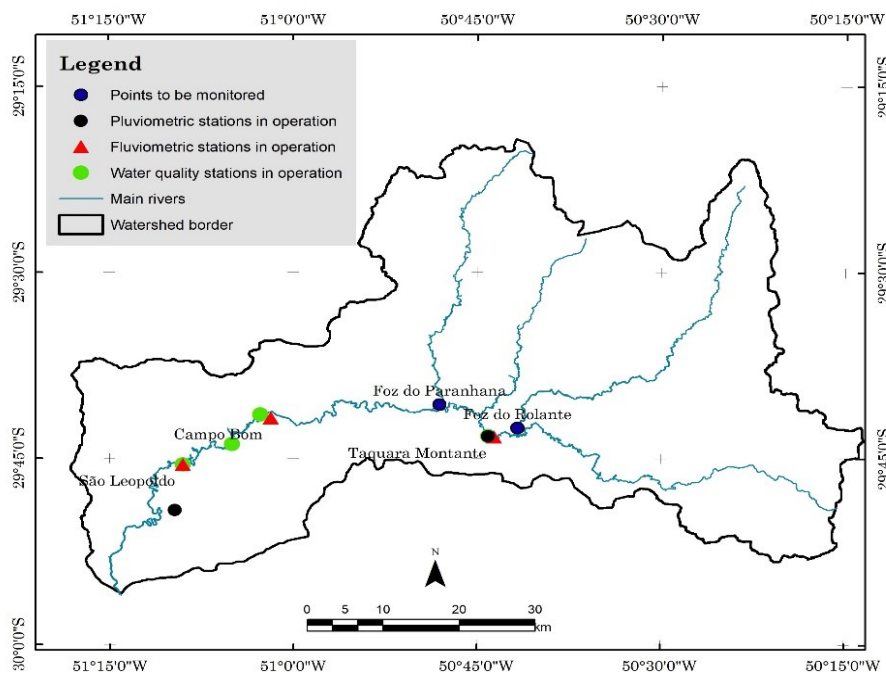
Figure 4 - Monitoring stations scattered along the Sinos River basin that are actually in operation and with data available for download at < http://www.snirh.gov.br/hidroweb >.
