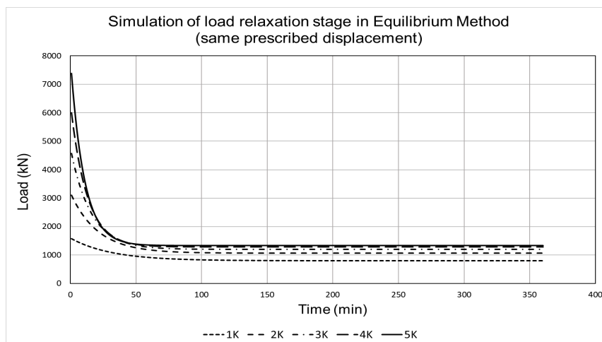
Figure A2. Simulation of load relaxation stage in Equilibrium Method, same prescribed displacement.
