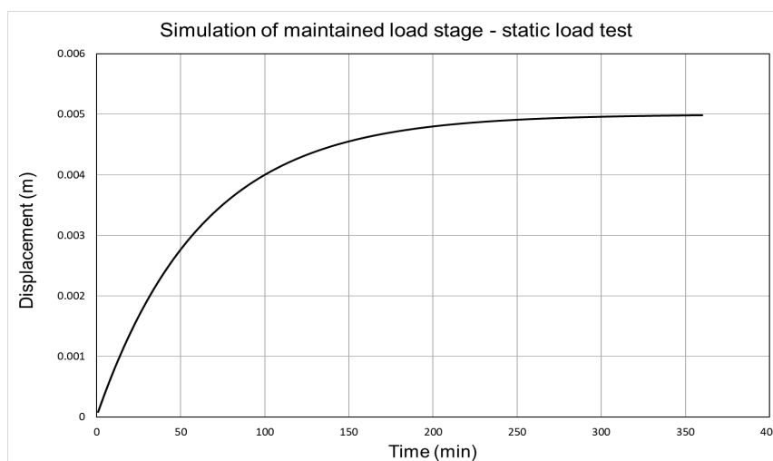
Figure A1. Simulation of (incremental) maintained load stage, conventional static load test.
