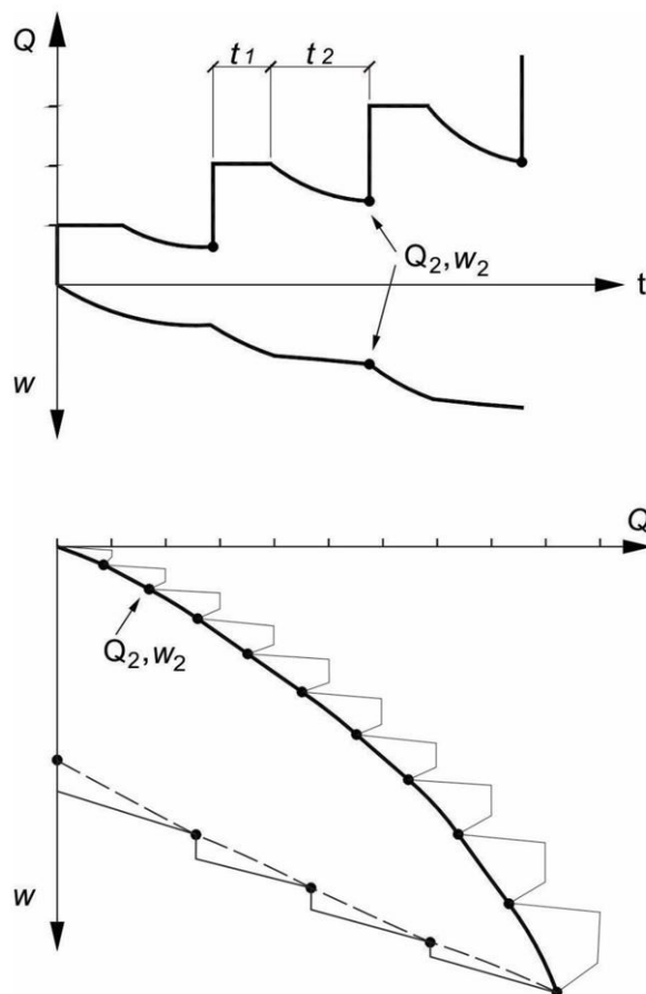
Figure 3. Typical graphs produced in the application of the Equilibrium Method.
