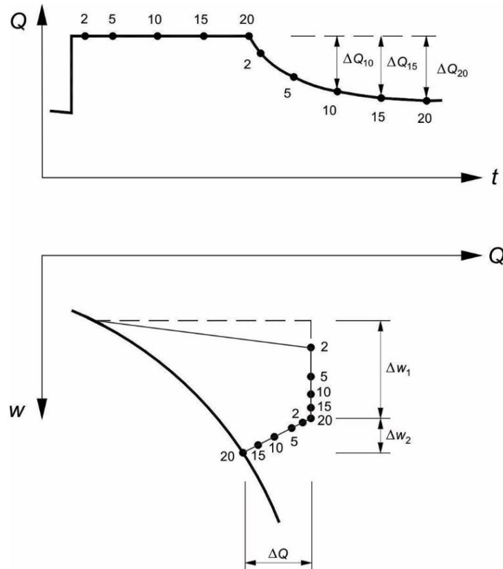
Figure 8. Details of a loading stage – Equilibrium Method – with reading times (in min) indicated.
