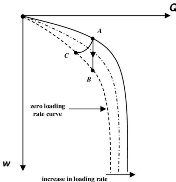
Figure 2. Possible load ( Q ) vs. displacement ( w ) curves in load tests and paths to reach the zero loading rate curve (Martins, 2006).
