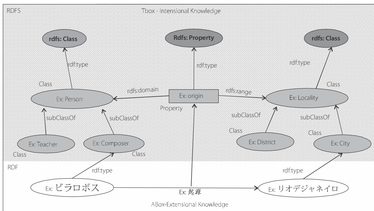
Figure 1. Intensional x Extensional Knowledge.
