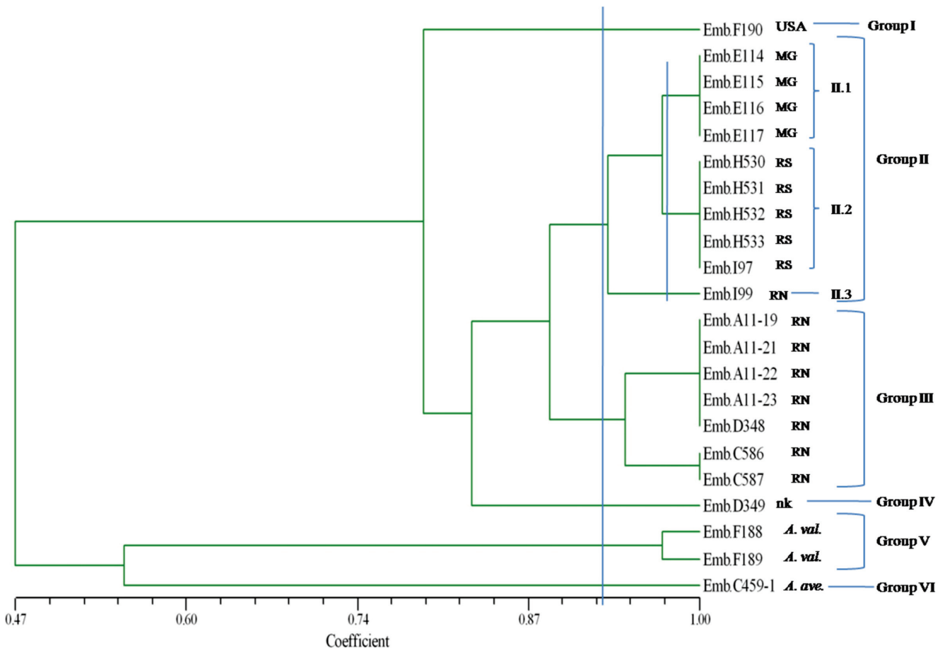
FIGURE 2 - Dendrogram constructed by comparing fingerprints of Acidovorax citrulli , A. avenae and A. valerianellae strains, obtained by BOX-PCR. Emb.F190 is the A. citrulli type strain (CFBP 4459). nk: Original location not known. A. val. : Acidovorax valerianellae . A. ave. : Acidovorax avenae .
