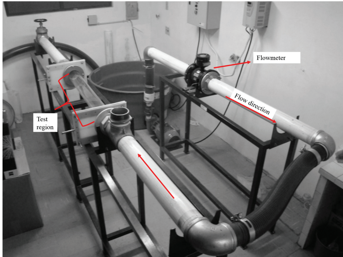
Figure 1. Experimental apparatus of swimming capacity showing the test region and flow direction.
