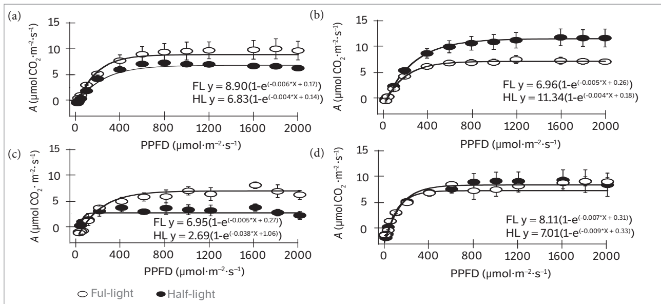
Figure 1. Light response curves of net photosynthesis ( A ) in function of photosynthetic photon flux density (PPFD) of Pachira aquatica (a,c) and Sterculia foetida (b,d) plants at 153 (phase I – a,b) and 410 days (phase II – c,d) under controlled conditions (constant temperature at 25°C and relative humidity at 68%) exposed to 1,000 (half-light - HL) and 2,000 \mu\text{mol}\cdot\text{m}^{-2}\cdot\text{s}^{-1} (full-light - FL) irradiance ( n = 3 \pm \text{SE} )
