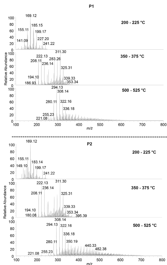
Figure 1. ESI(-) FT-ICR mass spectra of P1 and P2 of the distillate cuts.
